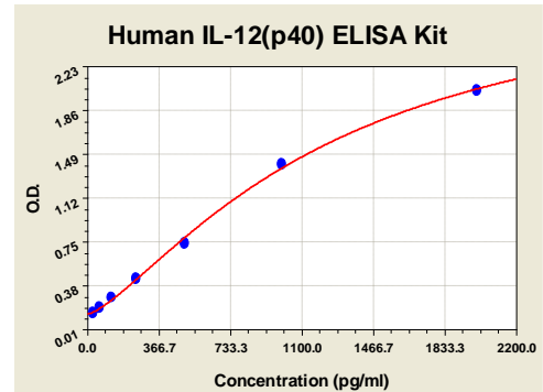
Figure 1: IL-12 (P40) Standard Curve. Using the Human IL-12 (P40) ELISA Kit, O.D. data was graphed against IL-12 (P40) protein concentration. The TMB reaction was incubated at 37° C for 30 min.
